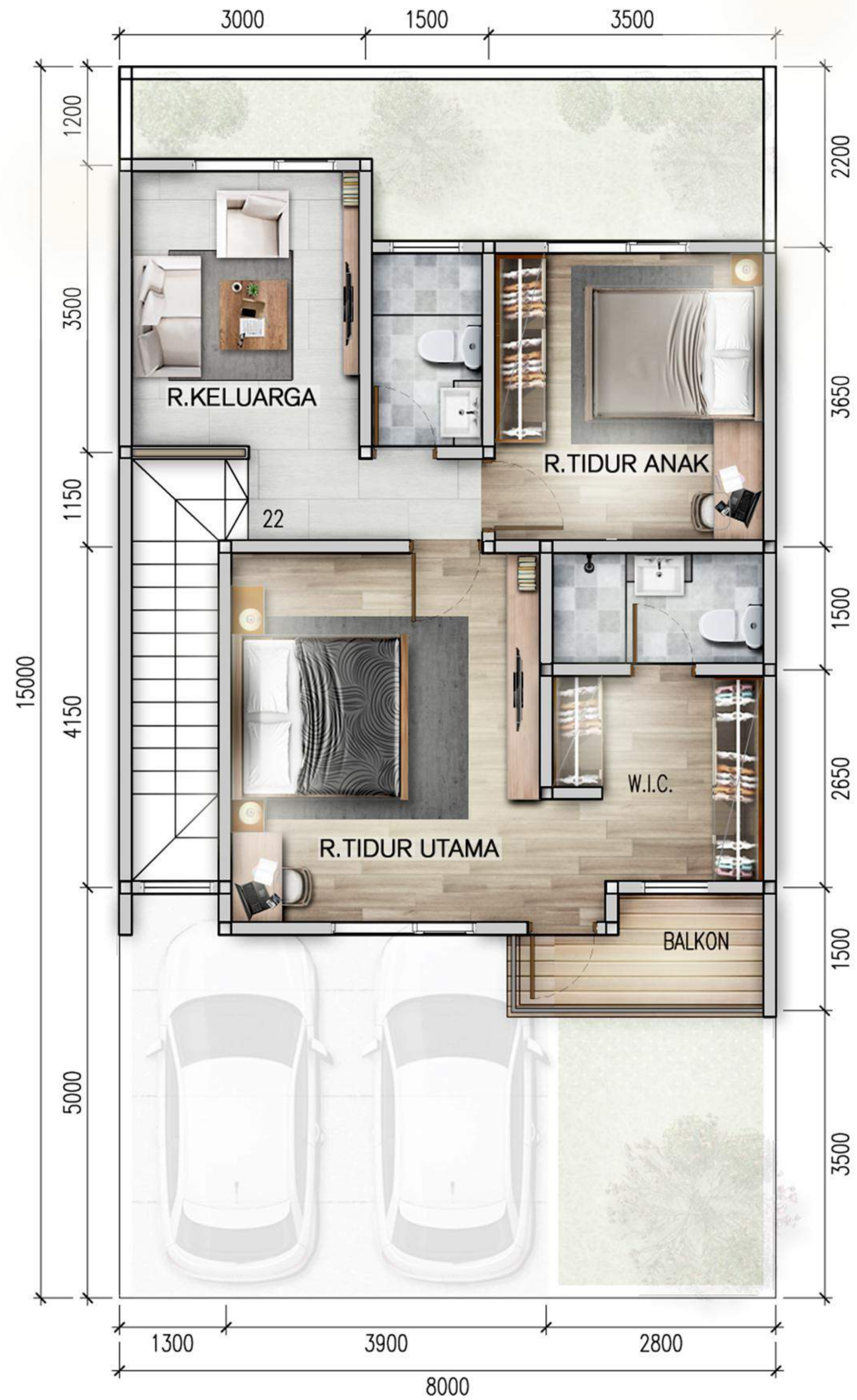
1 DENAH LT.DUA - SKALA 1:100 (72m 2 )
