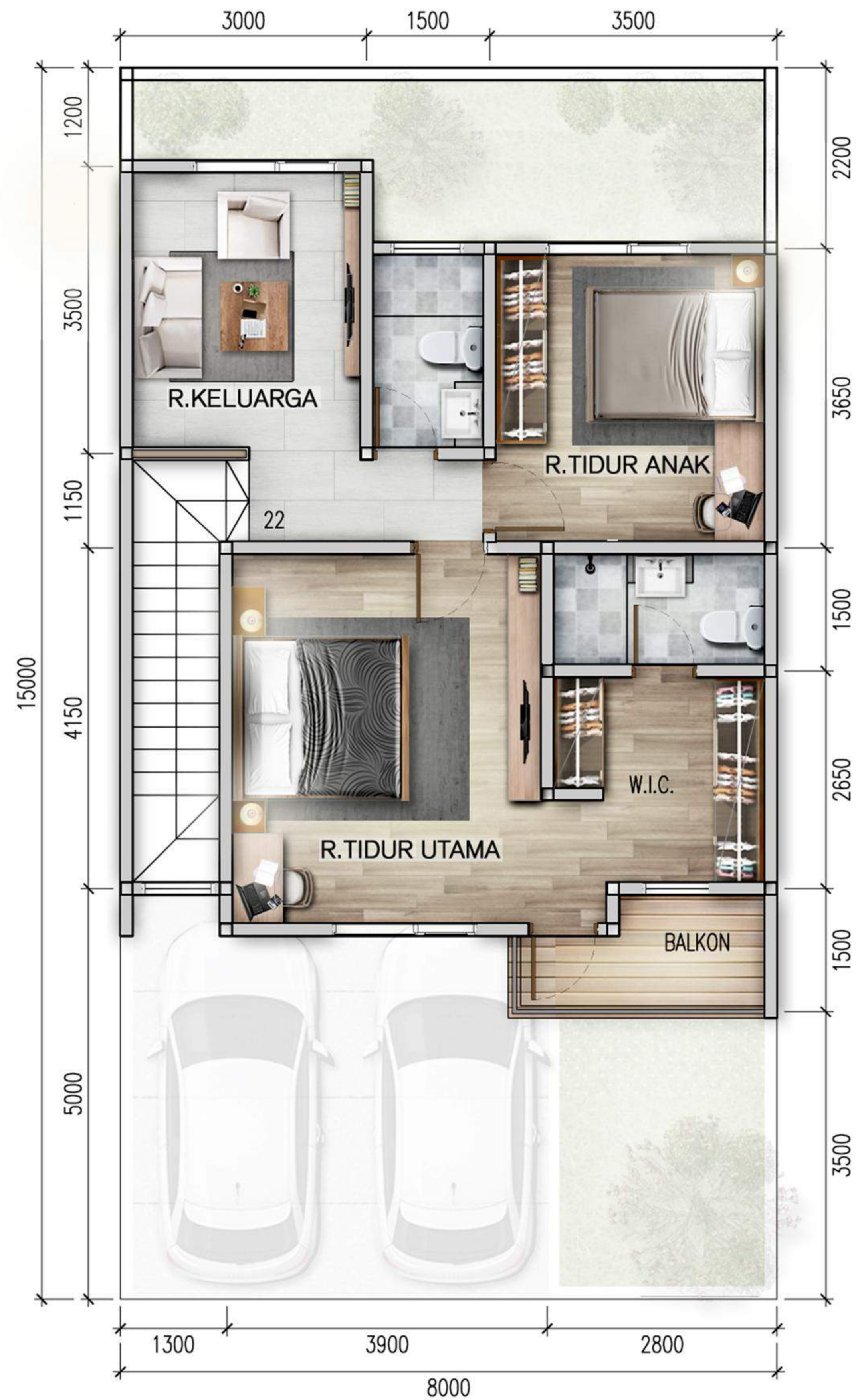
1 DENAH LT.DUA SKALA 1:100 (71m 2 )
