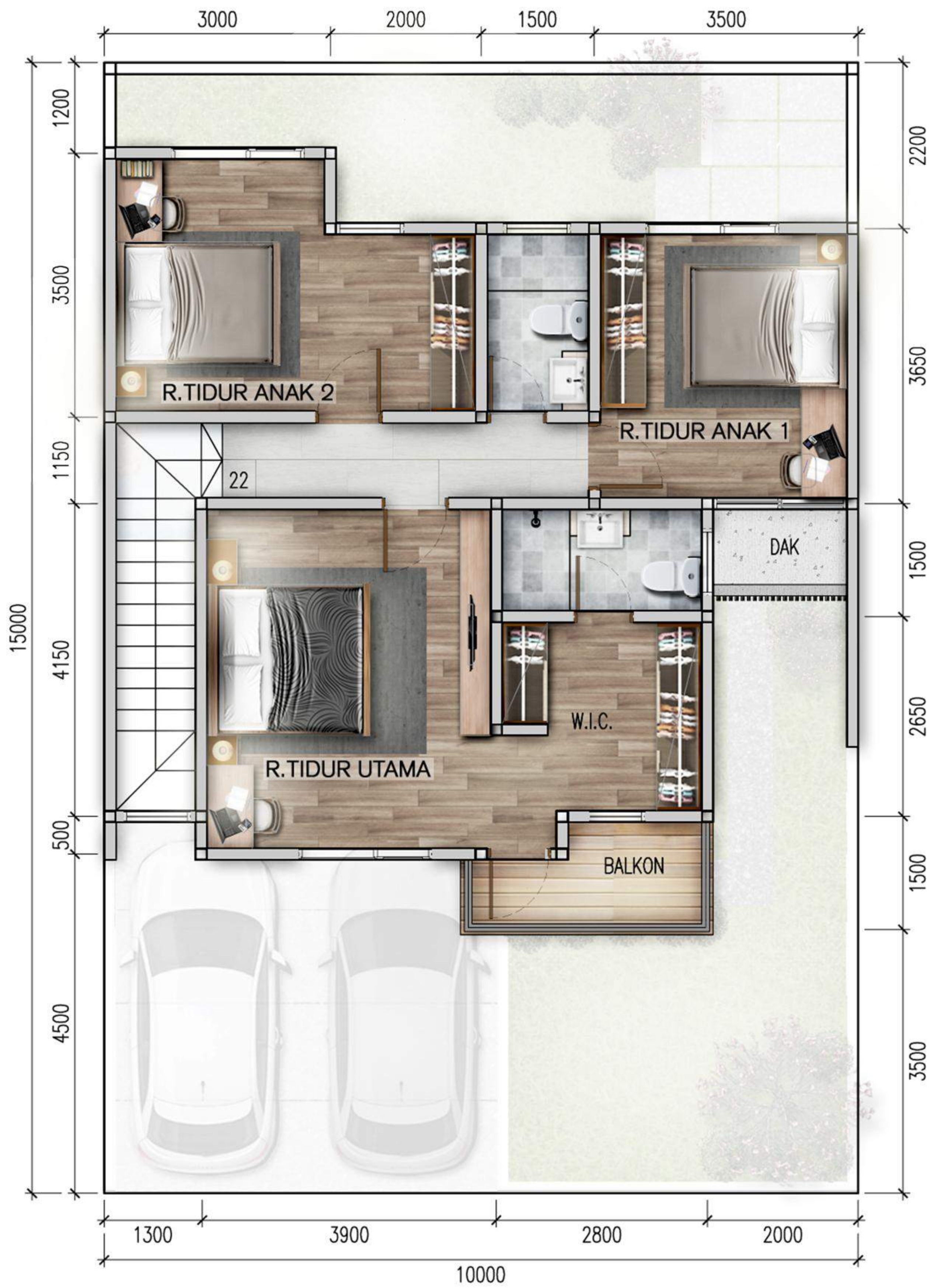
1 DENAH LT.DUA SKALA 1:100 (80m 2 ) HOOK
