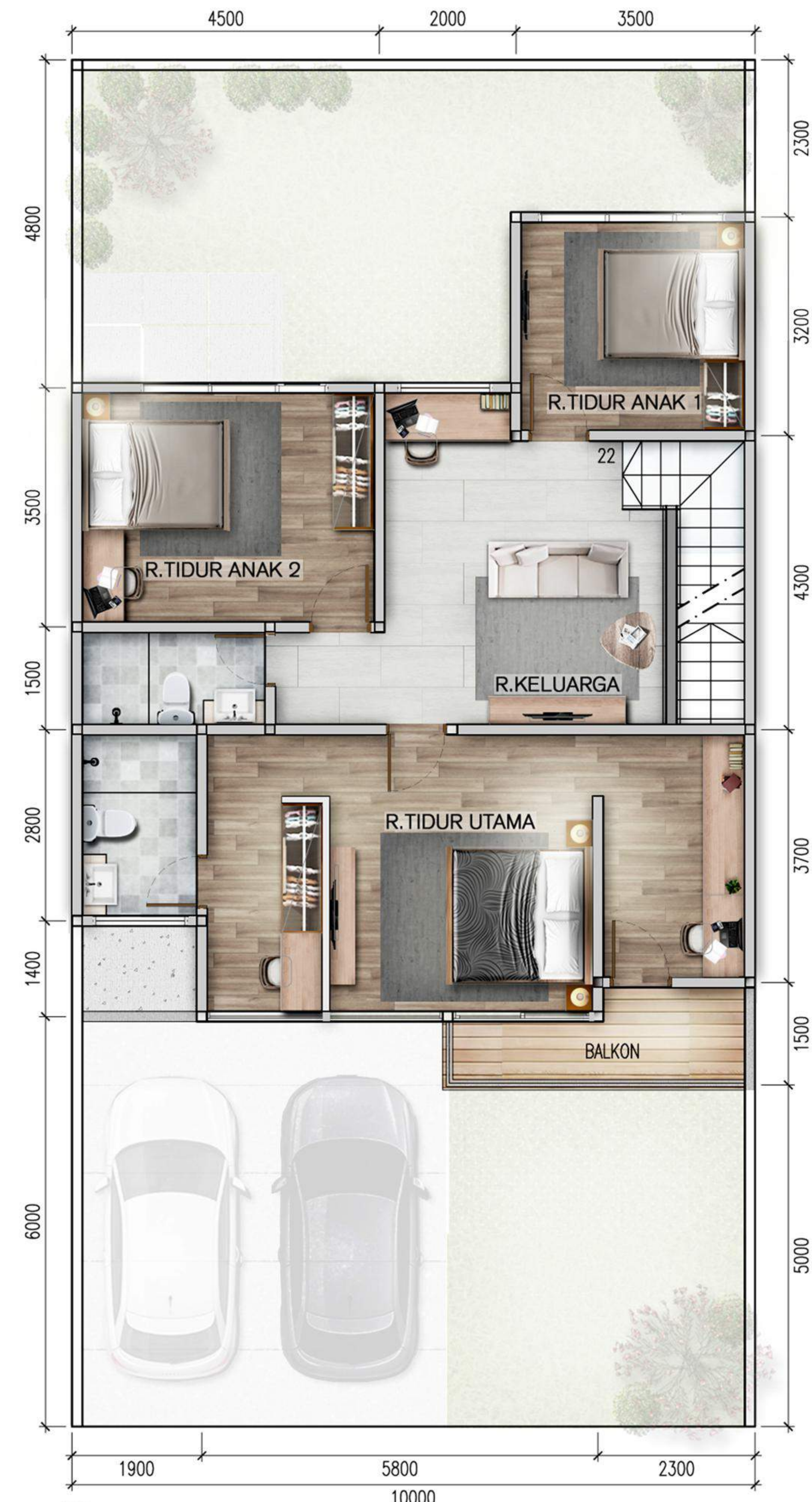
1 DENAH LT. DUA SKALA 1:100 (102m 2 )
