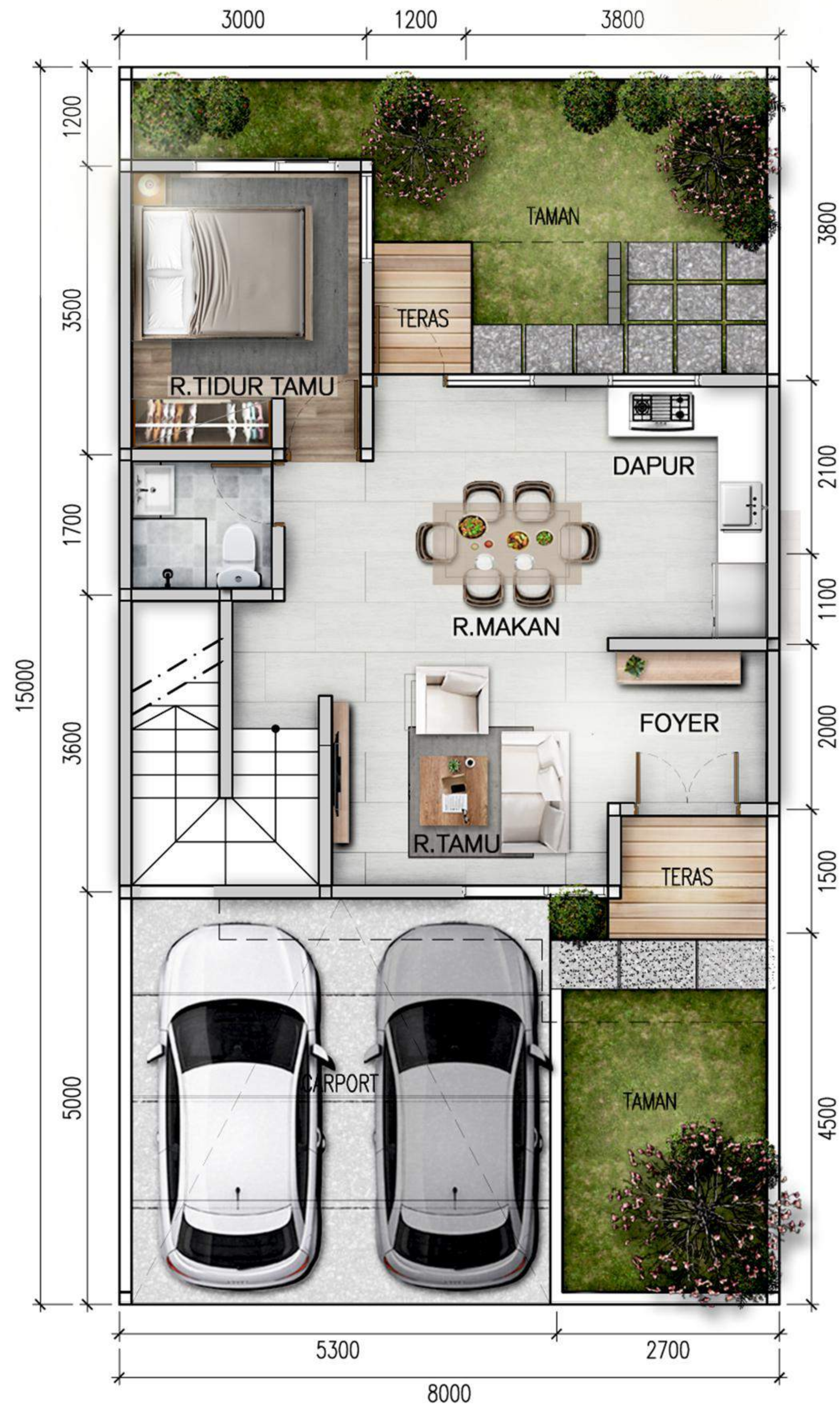
1 DENAH LT.SATU - SKALA 1:100 (60m 2 )
